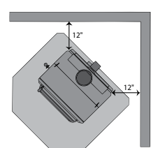
Corner Installation
