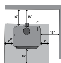
Standard Installation
